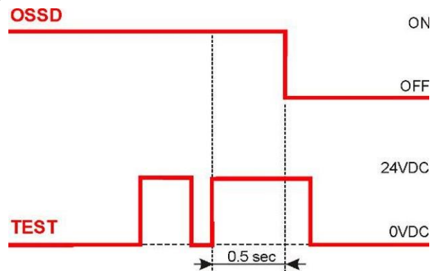
Fig 36 - Test timings
