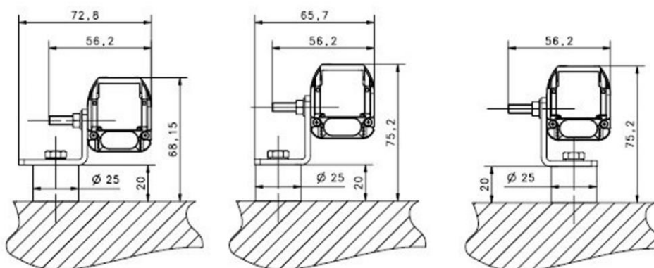
Fig 47 - Angled fixing bracket + Antivibration support
