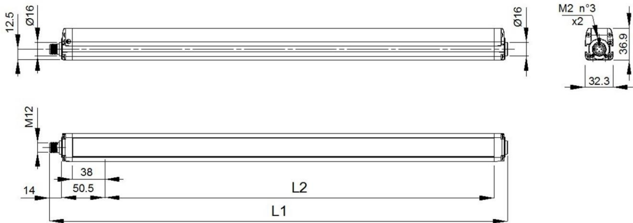
Fig 42 - Dimensions (mm)
