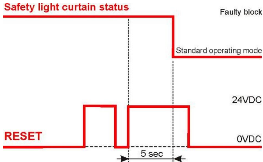
Fig 37 - Reset timings
