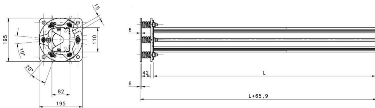
Fig 58 - Mounting
