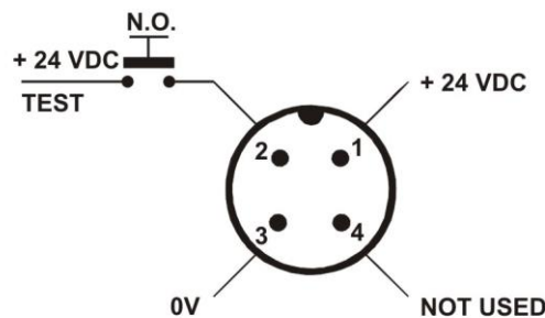
Fig 28 - Emitter
