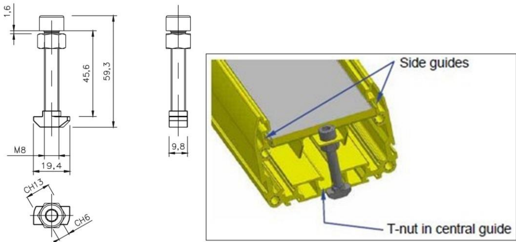
Fig 63 - Mounting kit
