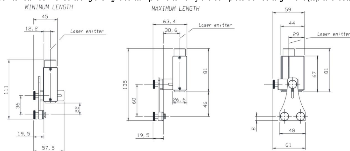
Fig 68 - Dimensions (mm)
