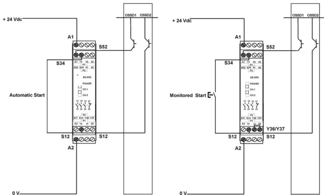
Fig 29 - Connection to SE-SR2 Safety Relays
