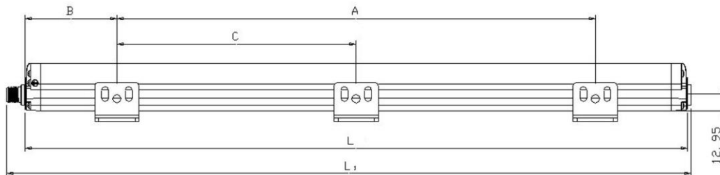
Fig 24 - Dimensions (mm)
