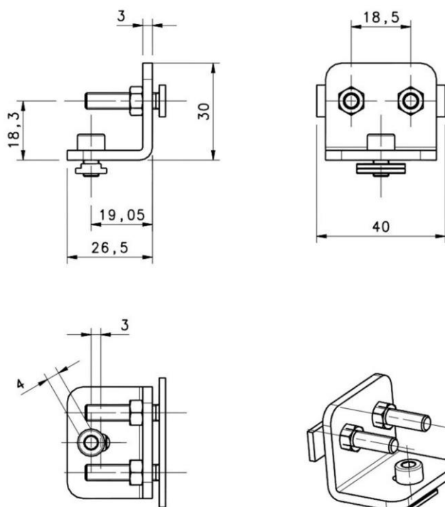
Fig 56 - Fixing kit
