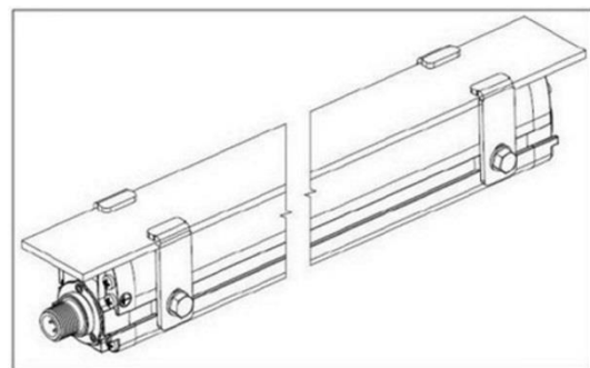
Fig 67 – Mounting kit
